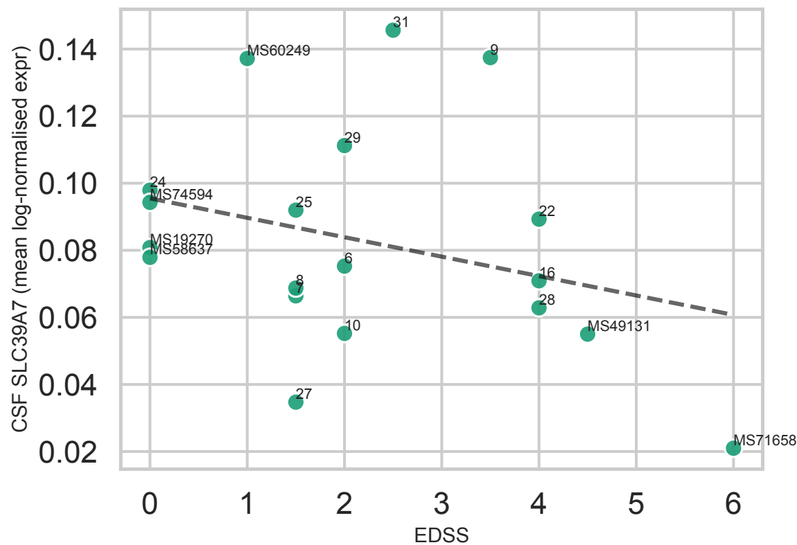
C. CSF SLC39A7 ( \rho=-0.34 , p=0.160 , \text{padj}=0.690 ) N=19
