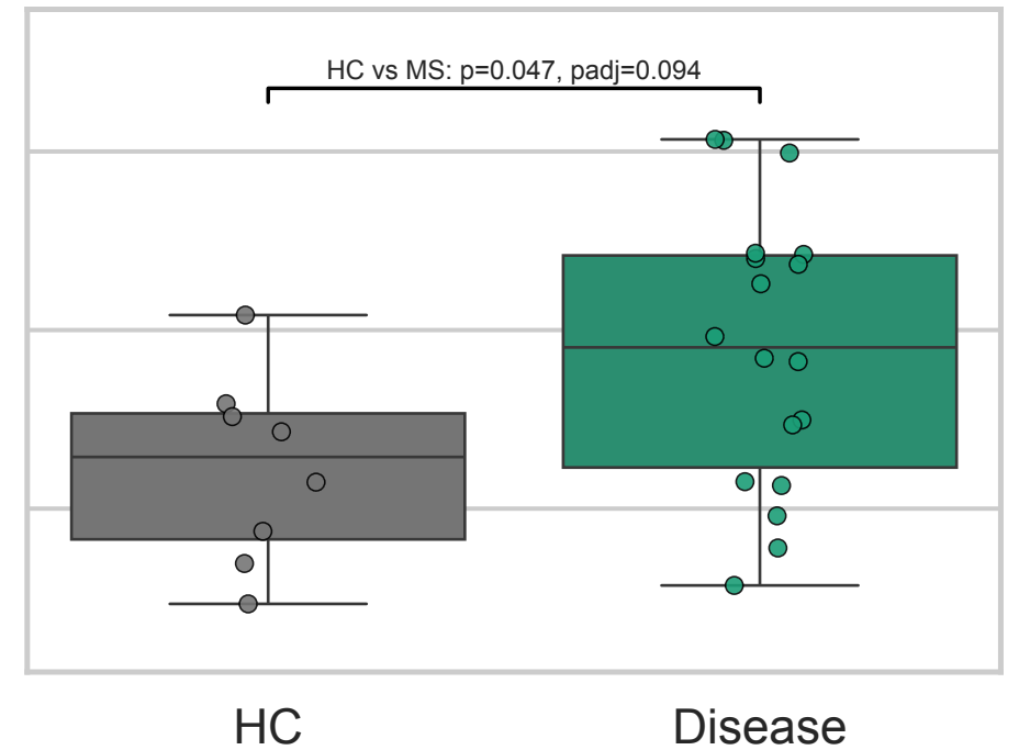
D. PB CXCR3+ B cells (signed)
