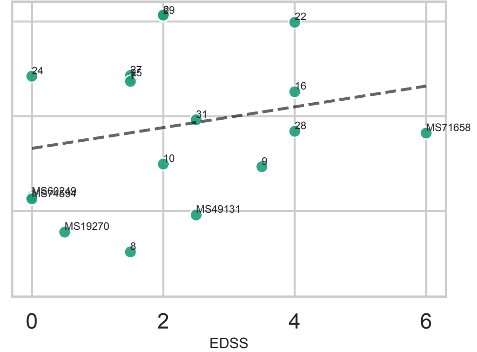
B. PB CXCR3+ B cells (signed) p=0.17 , p=0.494 , \text{padj}=0.494
