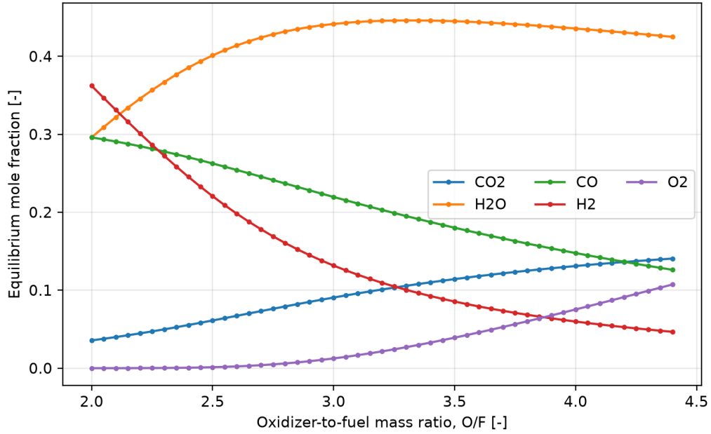
Figure 4: Major product mole fractions at chamber equilibrium.
