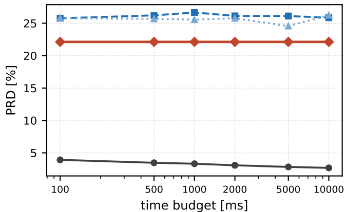
Dynasearch
