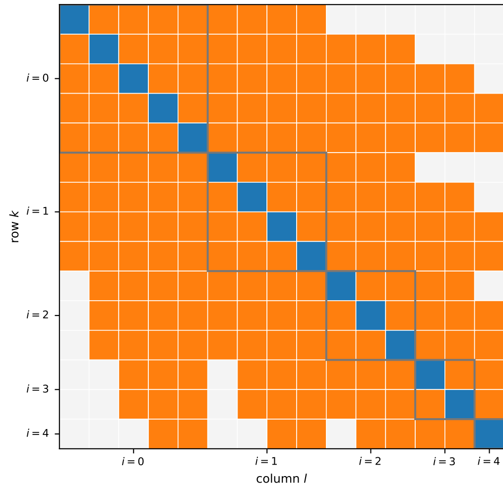
(a) Full Dynasearch QUBO, n = 6 , K = 15
