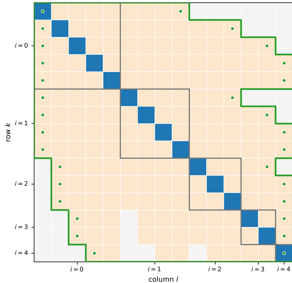
(b) Envelope curve: \mathcal{O}(K) memory suffices
