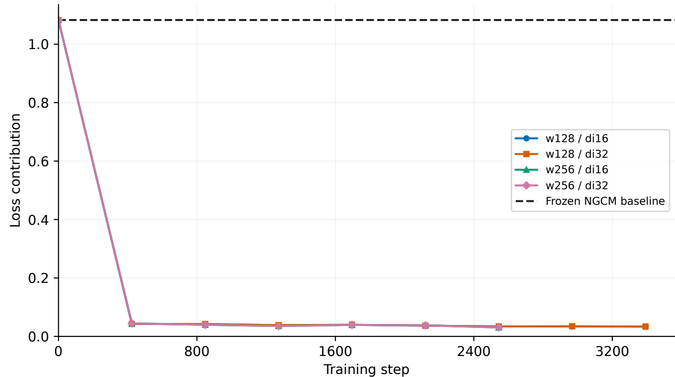
Current training loss v2 (6 h) — Geopotential Same v2-trained checkpoints; 2022 validation rescoring
