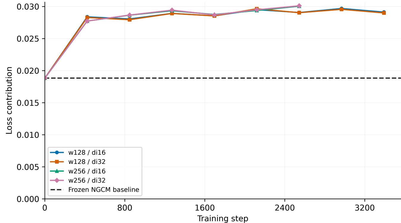
Current training loss v2 (6 h) — Specific humidity Same v2-trained checkpoints; 2022 validation rescoreing
