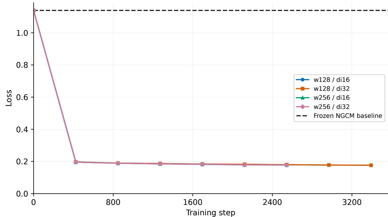
Current training loss v2 (6 h) — Total loss Same v2-trained checkpoints; 2022 validation rescoring
