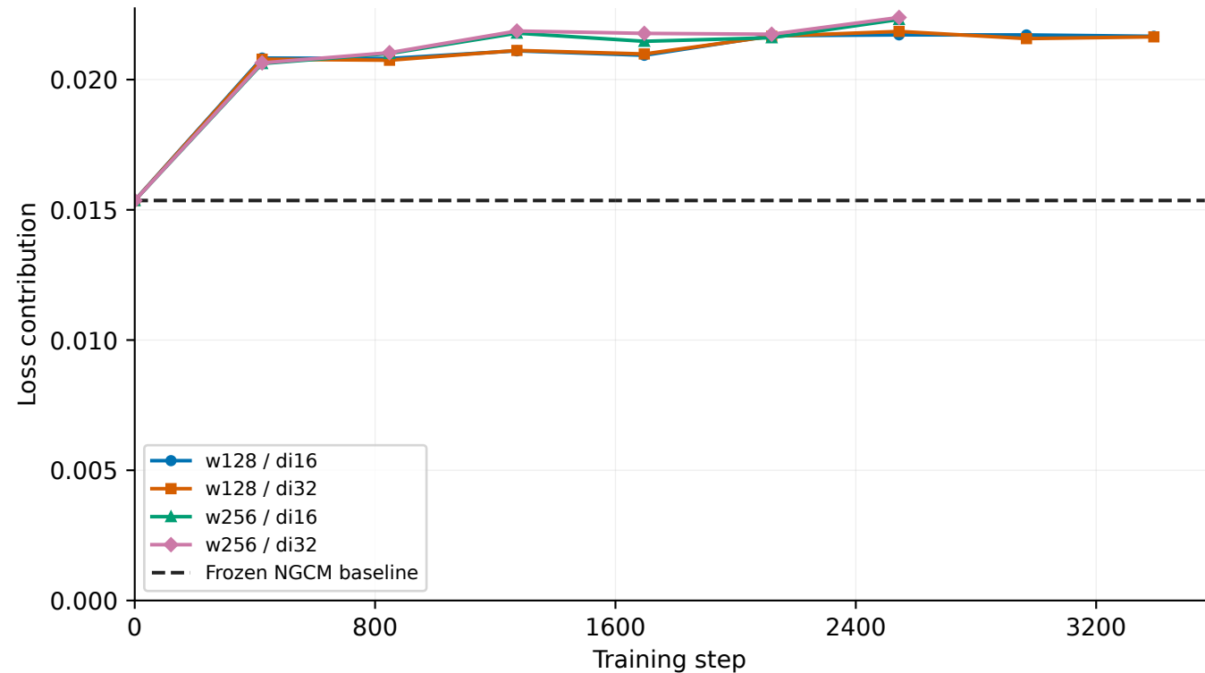
Current training loss v2 (6 h) — Eastward wind Same v2-trained checkpoints; 2022 validation rescore
