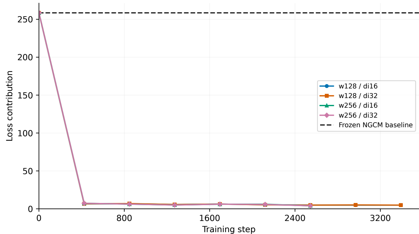
24 h simplified data MSE — Geopotential Same v2-trained checkpoints; 2022 validation rescoring
