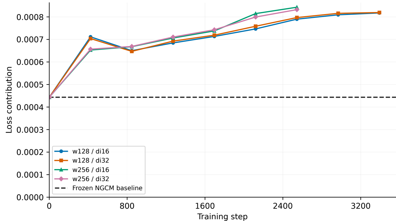
24 h simplified data MSE — Cloud liquid water Same v2-trained checkpoints; 2022 validation rescoring
