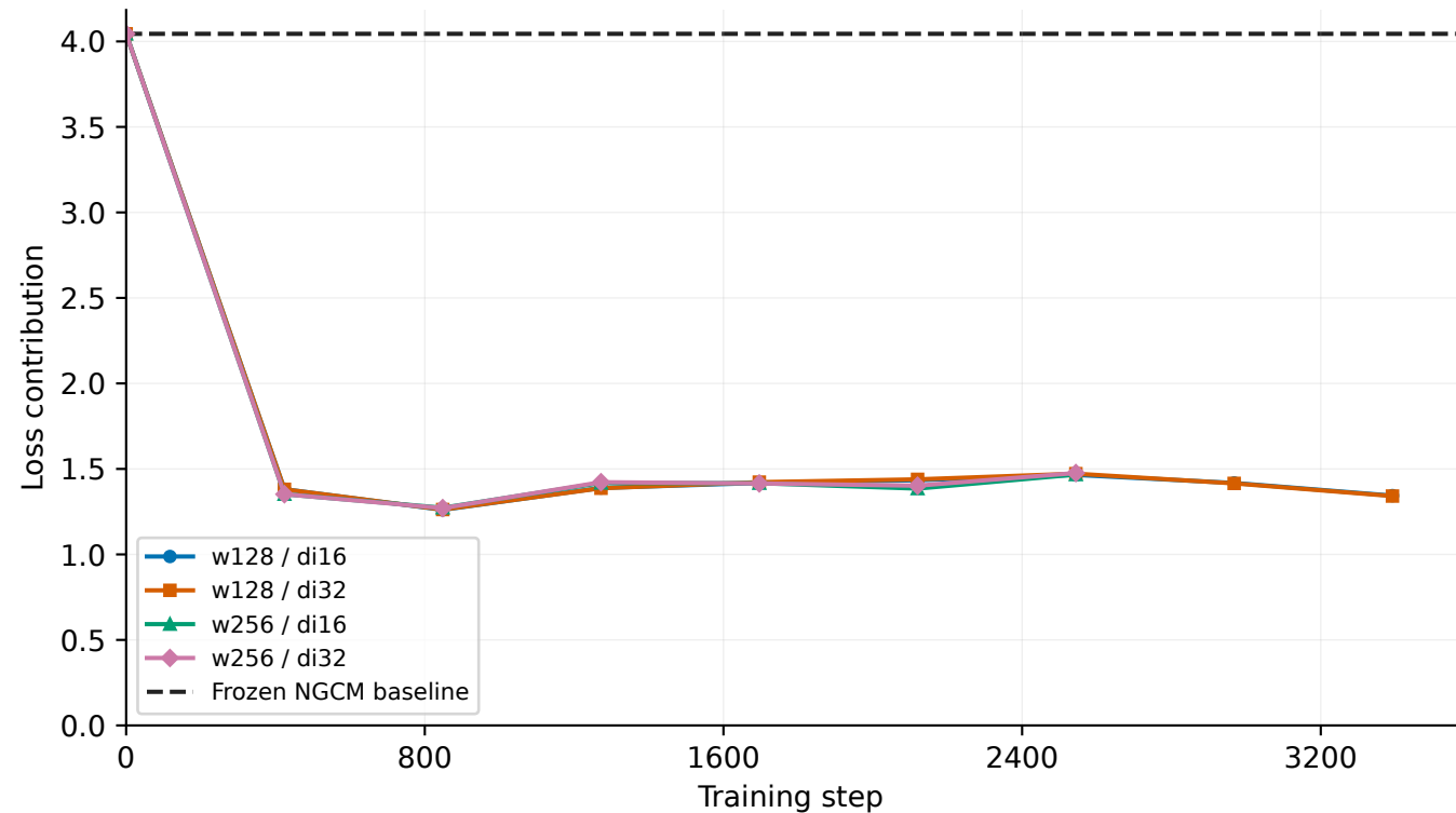
24 h simplified data MSE — Specific humidity Same v2-trained checkpoints; 2022 validation rescoring
