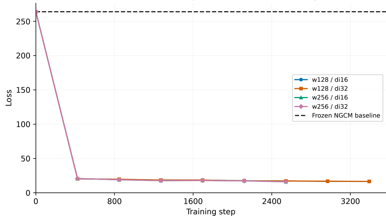
24 h simplified data MSE — Total loss Same v2-trained checkpoints; 2022 validation rescoring
