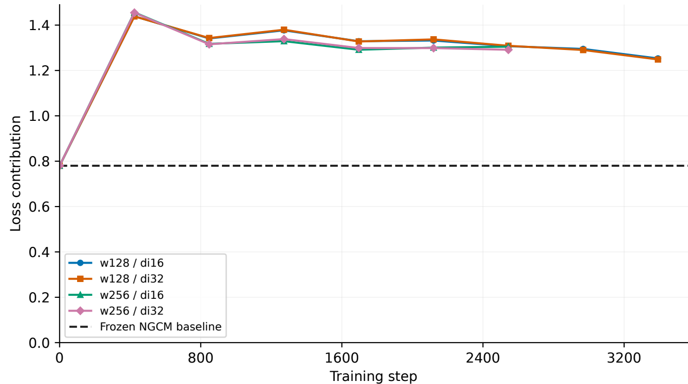
24 h simplified data MSE — Eastward wind Same v2-trained checkpoints; 2022 validation rescoring
