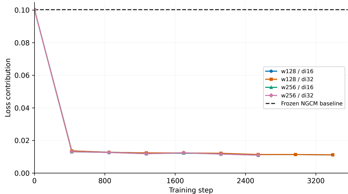
Original README loss (6 h) — Geopotential Same v2-trained checkpoints; 2022 validation rescoreing
