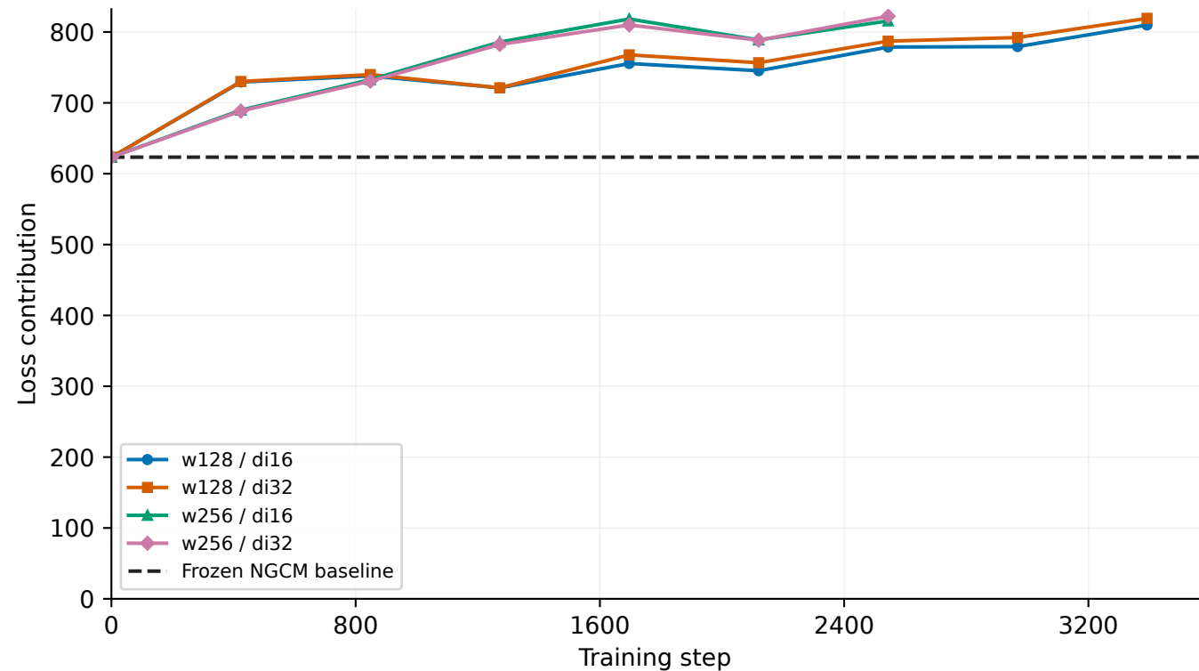
Original README loss (6 h) — Cloud ice Same v2-trained checkpoints; 2022 validation rescoring
