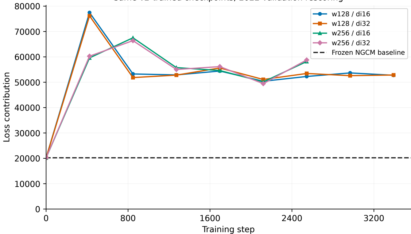
Original README loss (6 h) — Cloud liquid water Same v2-trained checkpoints; 2022 validation rescoring
