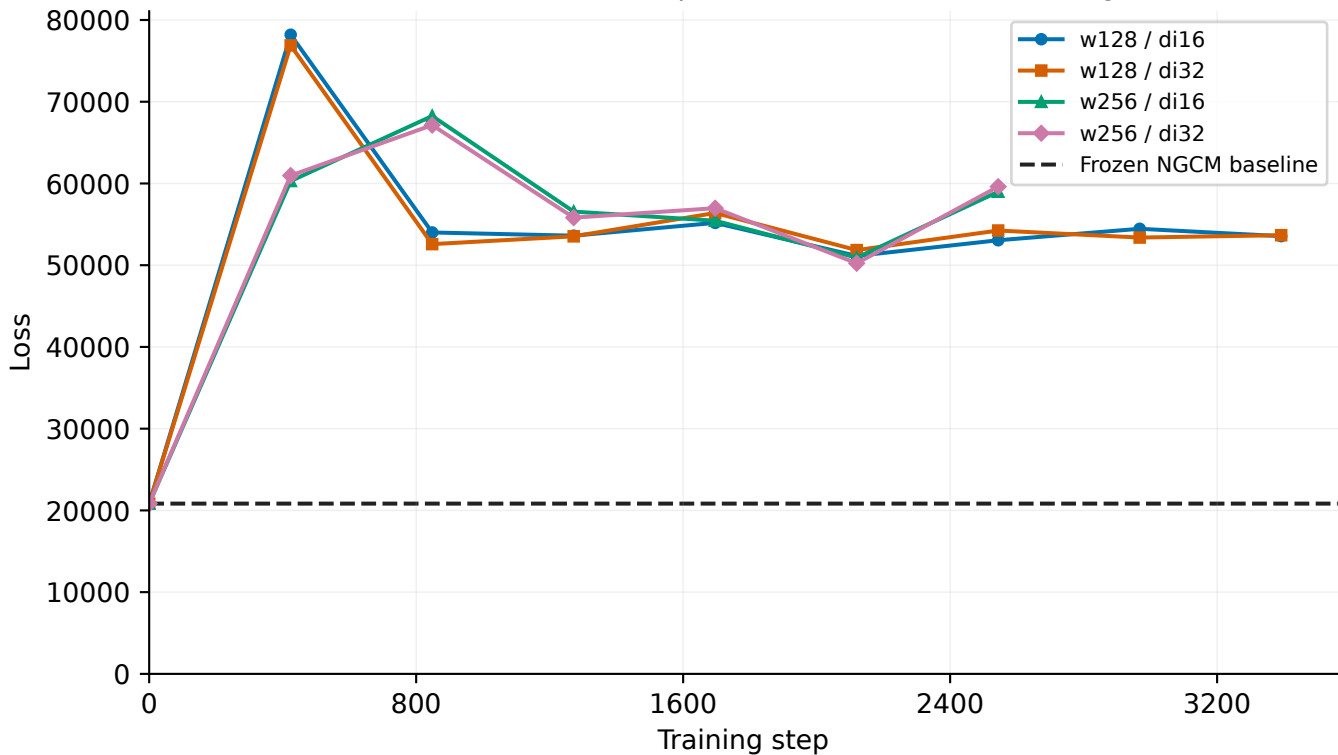
Original README loss (6 h) — Total loss Same v2-trained checkpoints; 2022 validation rescoreing
