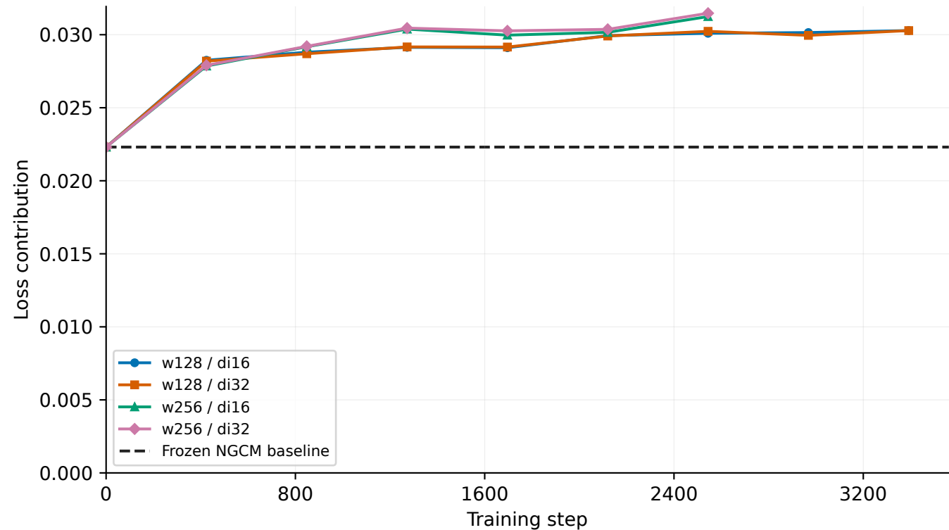
Original README loss (6 h) — Eastward wind Same v2-trained checkpoints; 2022 validation rescoreing
