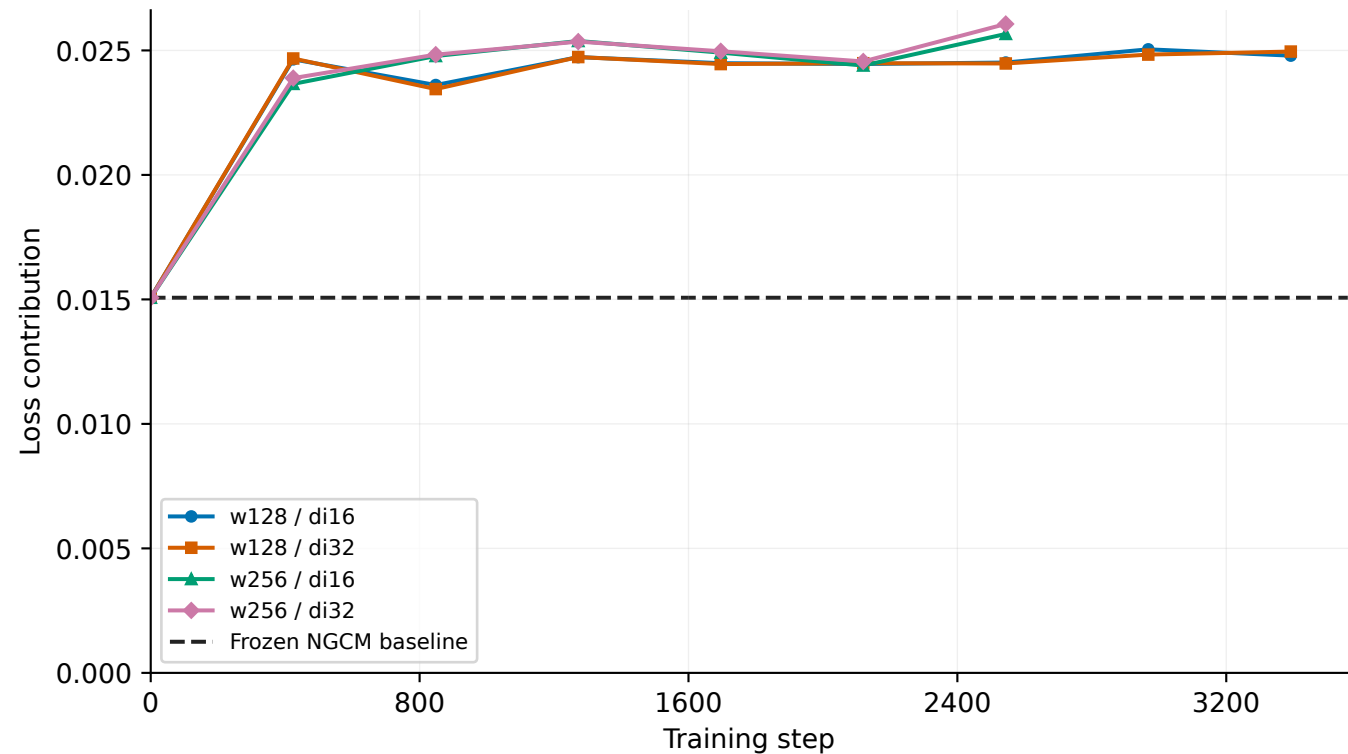
Original README loss (6 h) — Northward wind Same v2-trained checkpoints; 2022 validation rescore
