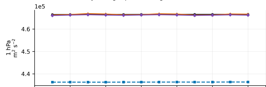
Physical geopotential: global area mean
