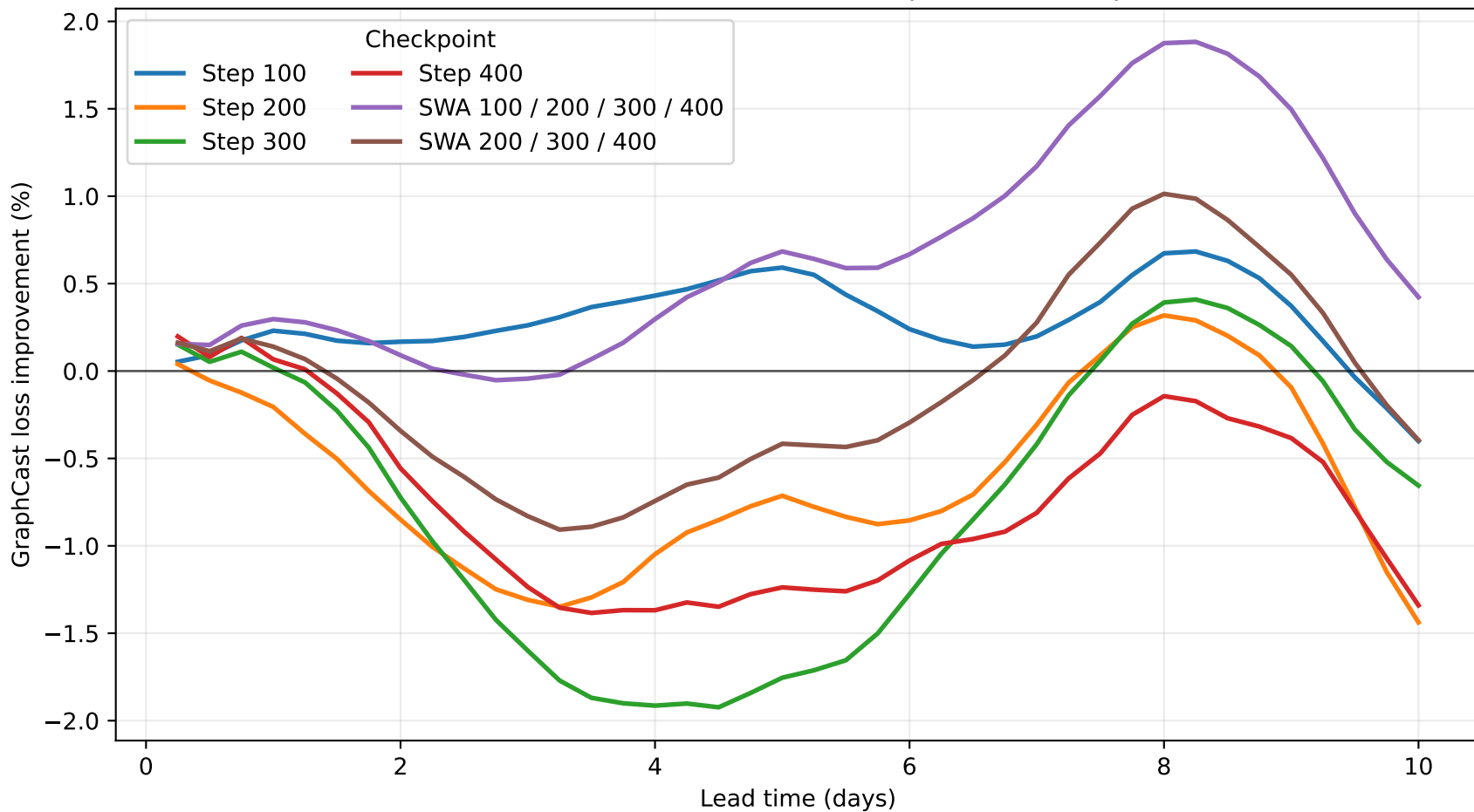
v24 res0.25 cold full-feedback: exact GraphCast loss improvement
