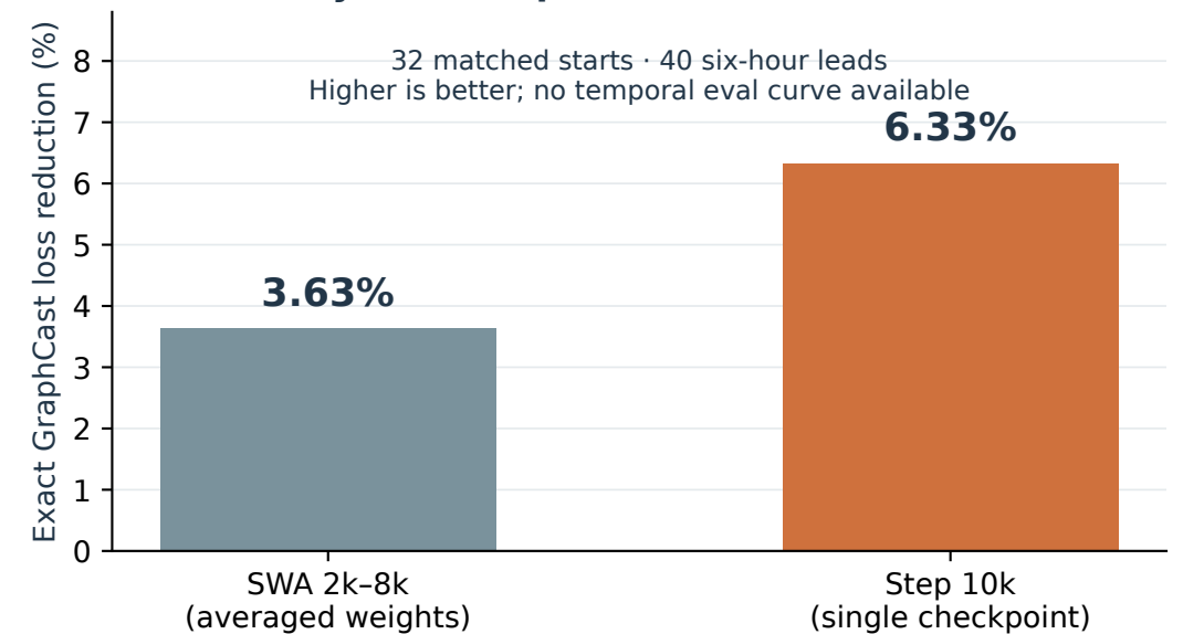
D Only two completed evaluation artifacts
