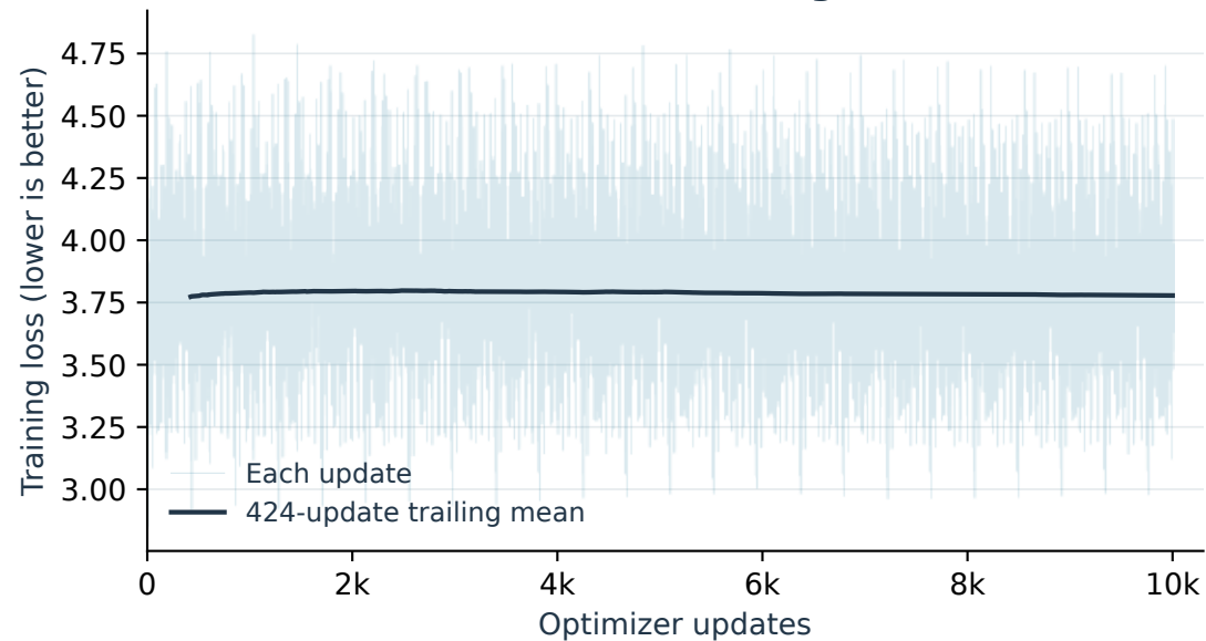
A Recorded training loss
