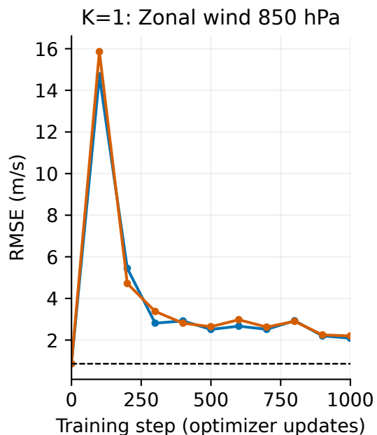
Physical forecast errors on the same 16 validation origins; lower is better K=2 averages squared errors over 6 and 12 h before taking the square root; dashed = frozen NGCM
