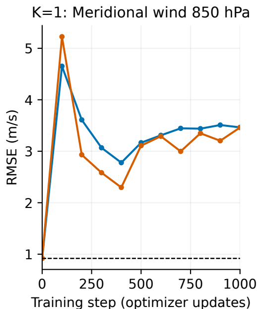
Physical forecast errors on the same 16 validation origins; lower is better K=2 averages squared errors over 6 and 12 h before taking the square root; dashed = frozen NGCM
