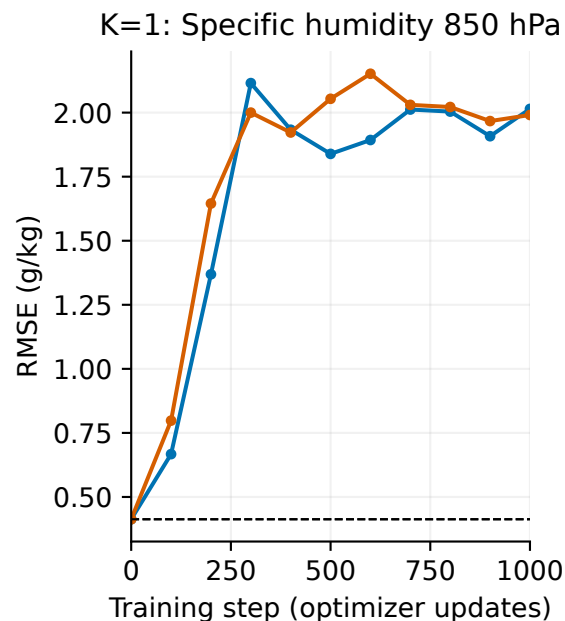
Physical forecast errors on the same 16 validation origins; lower is better K=2 averages squared errors over 6 and 12 h before taking the square root; dashed = frozen NGCM
