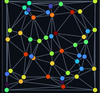
three-node cells over the domain
