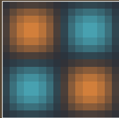
u_{22} \quad \lambda = 8\pi^2
