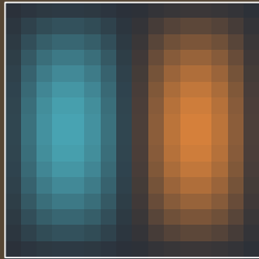
u_{21} \quad \lambda = 5\pi^2
