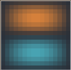
u_{12} \quad \lambda = 5\pi^2
