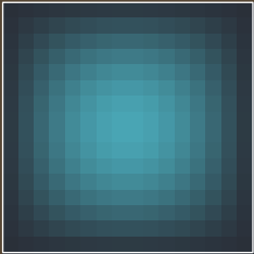
u_{11} \quad \lambda = 2\pi^2
