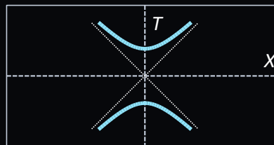
WAVE · HYPERBOLIC
