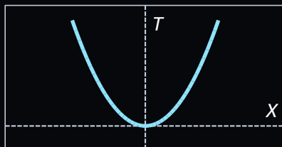
HEAT · PARABOLIC
