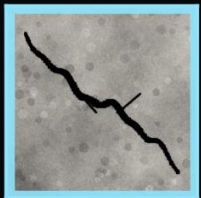
CLASSIFY
