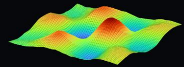
RMSE 0.032
