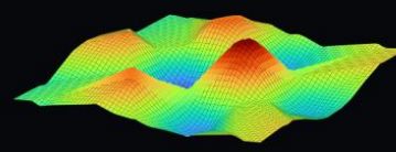
RMSE 0.050
