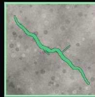
SEGMENT
