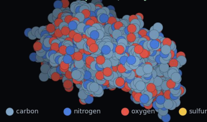
the folded protein, every atom
