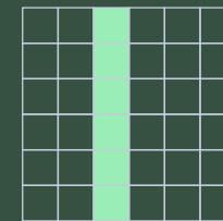
batch norm
