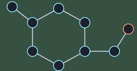
molecule
