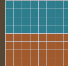
(1,2) \lambda = 5\pi^2
