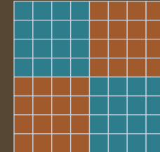
(2,2) \lambda = 8\pi^2
