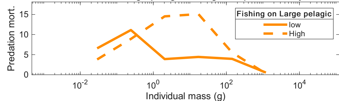
C. Effect of large pelagic fishing on squid mortality
