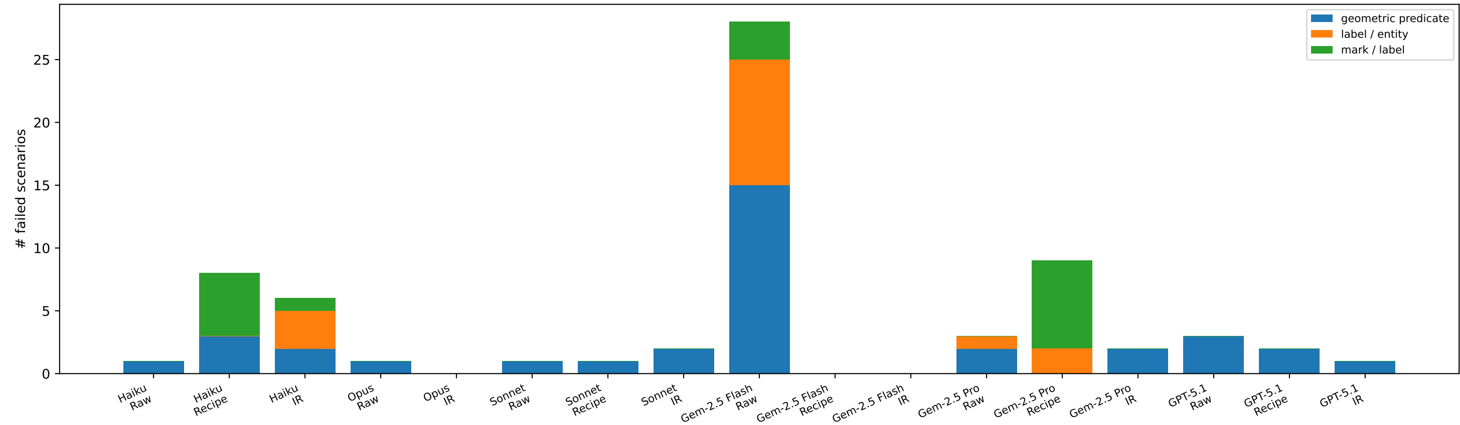
Failure modes by (model, strategy)
