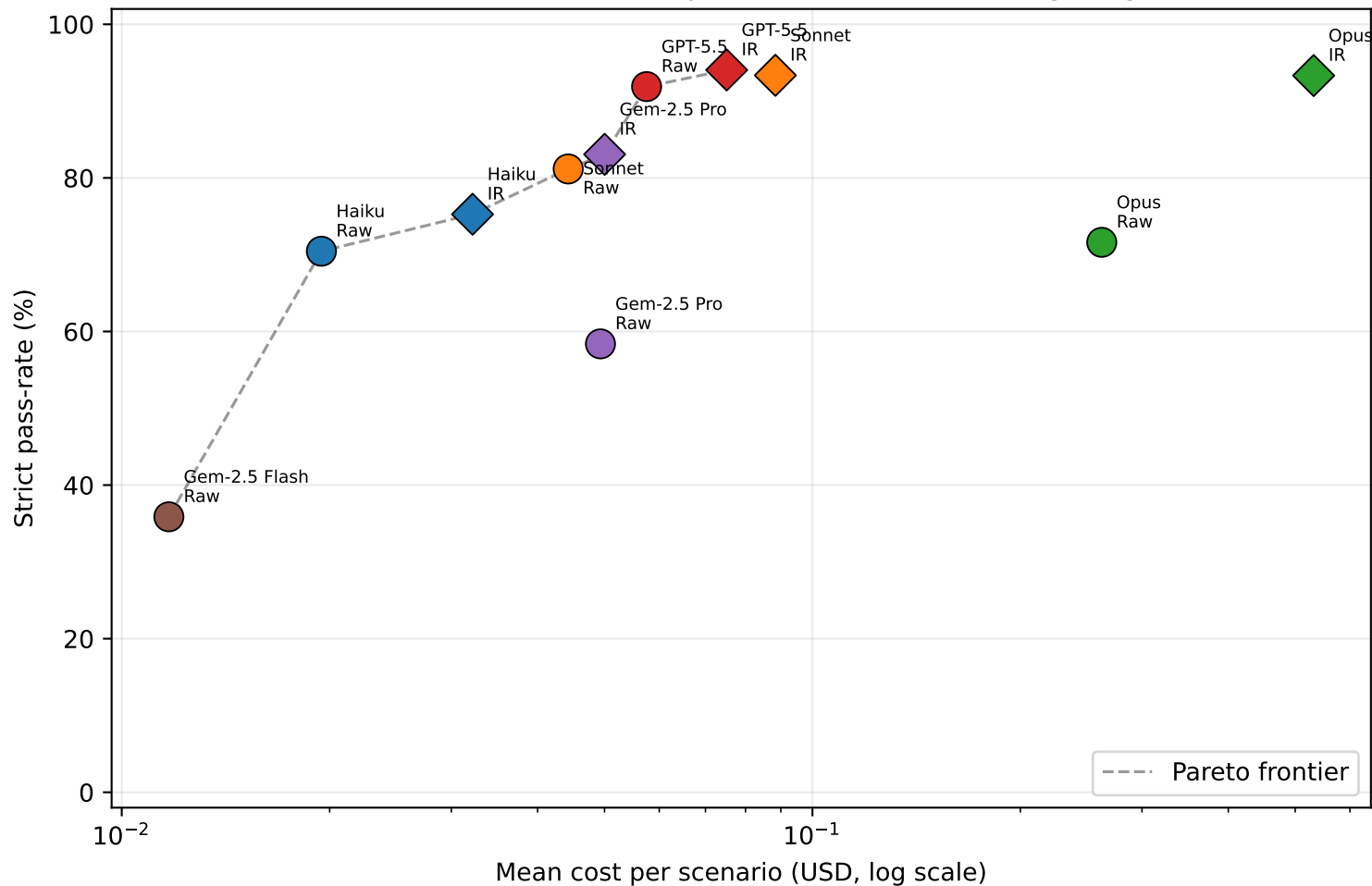
GeoGen leaderboard — pass-rate \times cost (strict gating)
