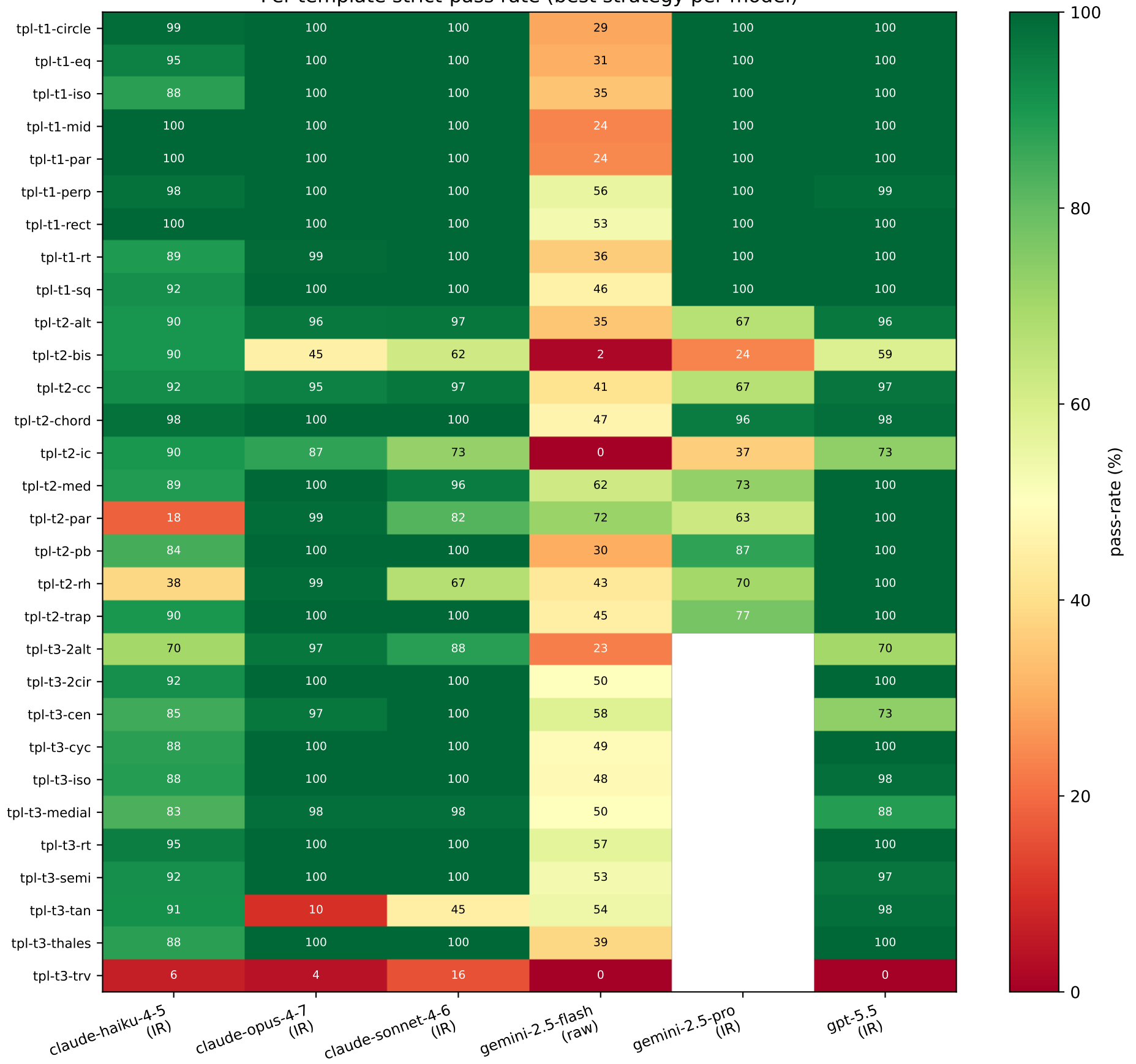
Per-template strict-pass rate (best strategy per model)
