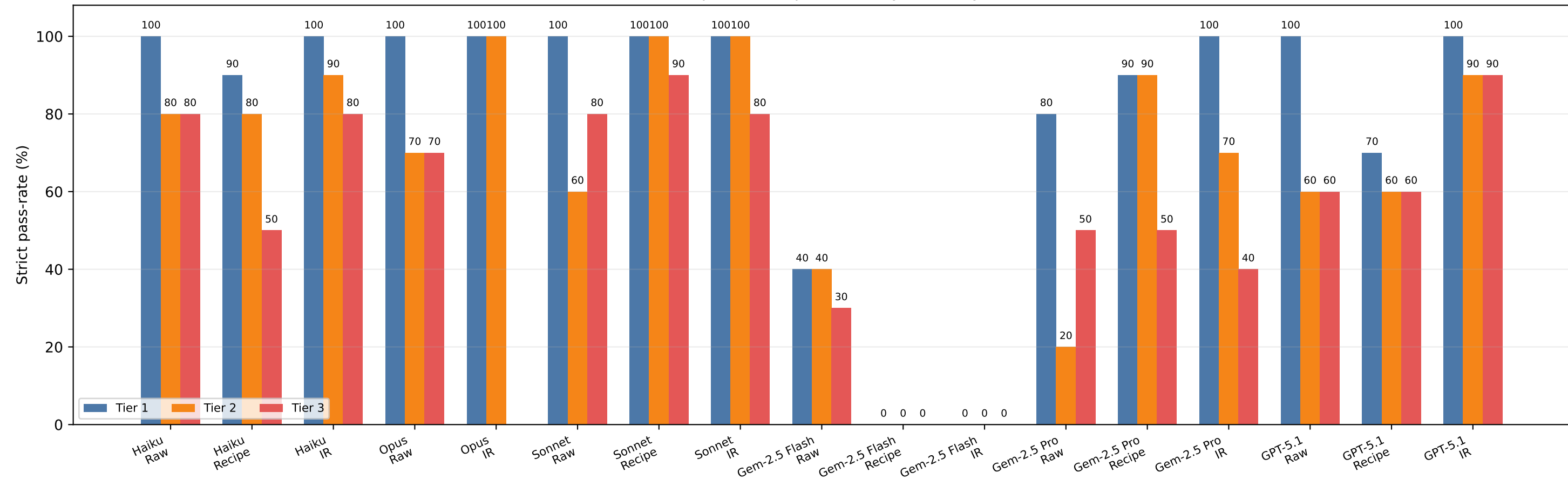
GeoGen pilot strict pass-rate by difficulty tier
