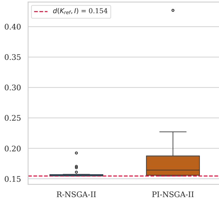
WeldedBeam
