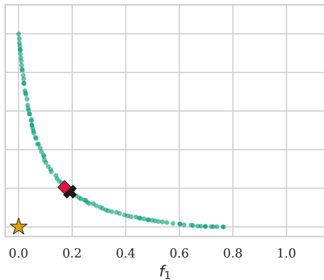
PI-NSGA-II (run #18)
