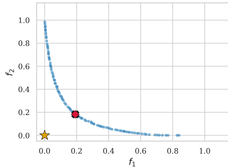
NSGA-II (run #16)
