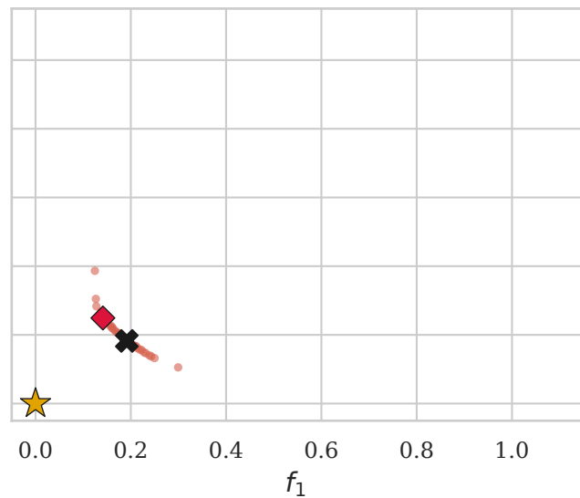
R-NSGA-II (run #17)
