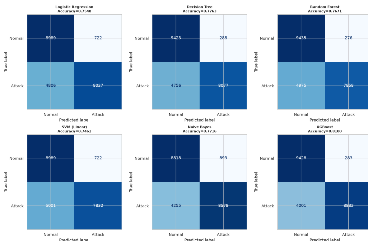
Figure 5. Confusion matrices for all six models on the test set. The large bottom-left cells are missed attacks (false negatives).
