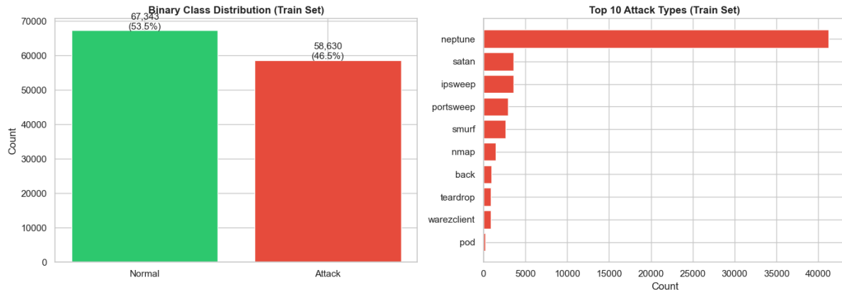
Figure 1. Binary class balance (left) and the ten most frequent attack types (right). neptune dominates.
