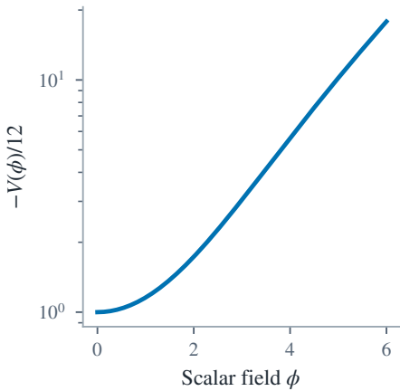
(a) Dilaton potential
