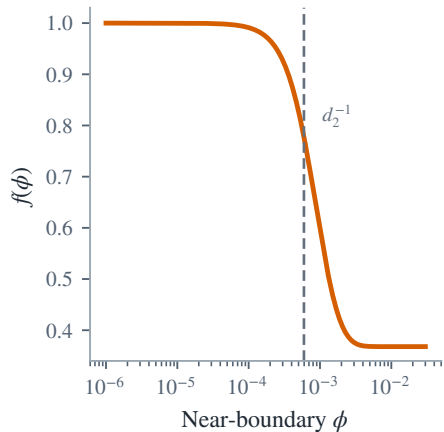
(c) UV boundary layer
