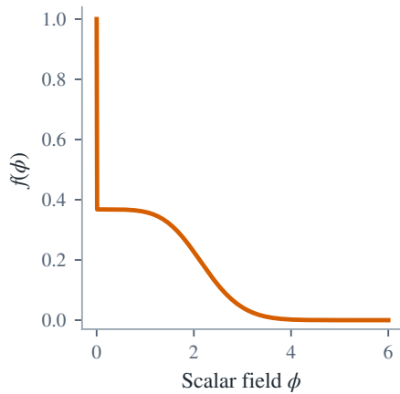
(b) Maxwell coupling
