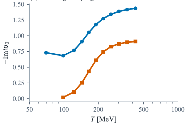
(b) Leading damping
