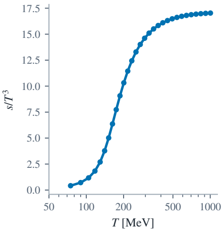
(a) Neutral entropy
