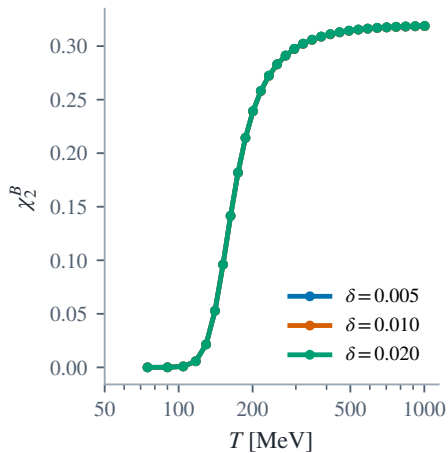
(b) Baryon susceptibility
