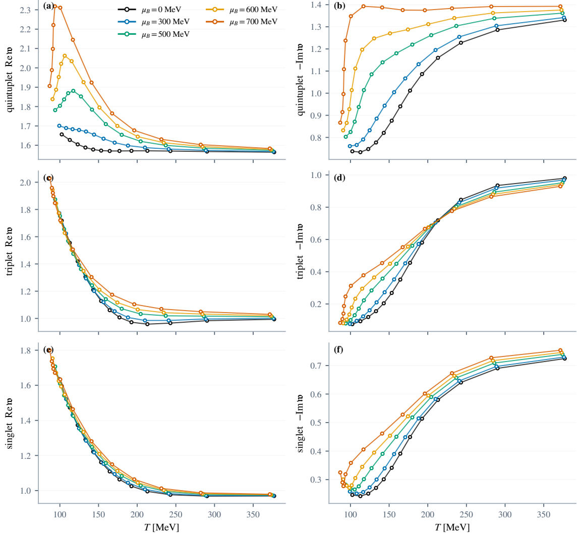
Figure 13. Independent numerical reproduction using the 2018 EMD parametrization. Rows show the quintuplet, triplet, and singlet; columns show \text{Re } \omega and -\text{Im } \omega versus temperature at five fixed chemical potentials. Open markers are source-factored collocation calculations and thin segments are piecewise-linear guides to the eye, not fitted or digitized published curves. Sixty-five backgrounds give 195 displayed QNM points. Independent shooting at the nine landmarks of table 8 supplies the quantitative cross-check. The reproduction validates the shared solver for a known parametrization; it does not imply universality between that model and PHA.
