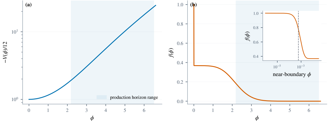
Figure 6. Exact MAP model kernels. Panel (a) shows the dilaton potential and panel (b) the Maxwell coupling; the light blue region marks the horizon-field range sampled by the production phase surface. The inset resolves the near-boundary coupling layer at \phi \sim d_2^{-1} . Curves are direct evaluations of the analytic parametrization, not fits or interpolations.
