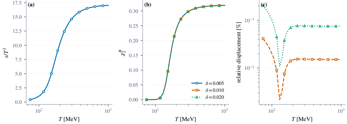
Figure 10. Reproduction and step-size stability of neutral thermodynamics. Panel (a) shows s/T^3 . Panel (b) shows \chi_2^B from eq. (D.10); color, marker, and line style redundantly encode the three charge steps. Panel (c) gives the relative displacement from the finest step in percent, rather than mixing absolute and relative scales. Symbols are calculated backgrounds and connecting segments only guide the eye. This equilibrium validation is independent of the finite-density critical and spinodal claims.
