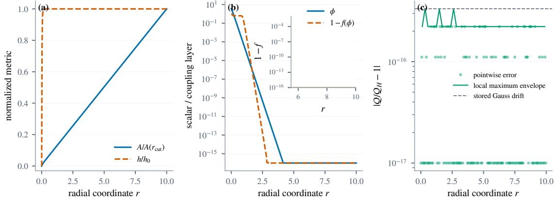
Figure 7. MAP critical background used by the homogeneous and coupled benchmarks. Panel (a) shows normalized metric functions. Panel (b) shows scalar decay and the Maxwell-coupling boundary layer, with an inset resolving its UV tail. Panel (c) displays the pointwise relative electric-flux error and its local maximum envelope rather than the nearly constant flux itself; the dashed line is the independently stored Gauss-drift diagnostic. The regular profiles and small relative error test the background input without relying on a QNM calculation.
