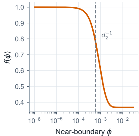
(c) UV boundary layer
