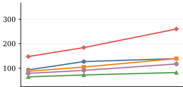
BoolQ
