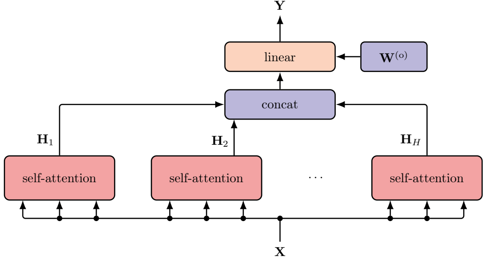
Figure 2.4: Multi-Head Attention.
