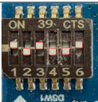
Figure 54. DSW1 – xSPI Boot Mode
