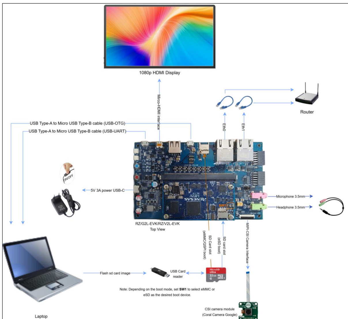
Figure 24. Complete setup for RZ/G2L-EVK & RZ/V2L-EVK
