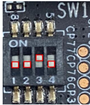
Figure 17. RS-G2L100 xSPI boot switch
