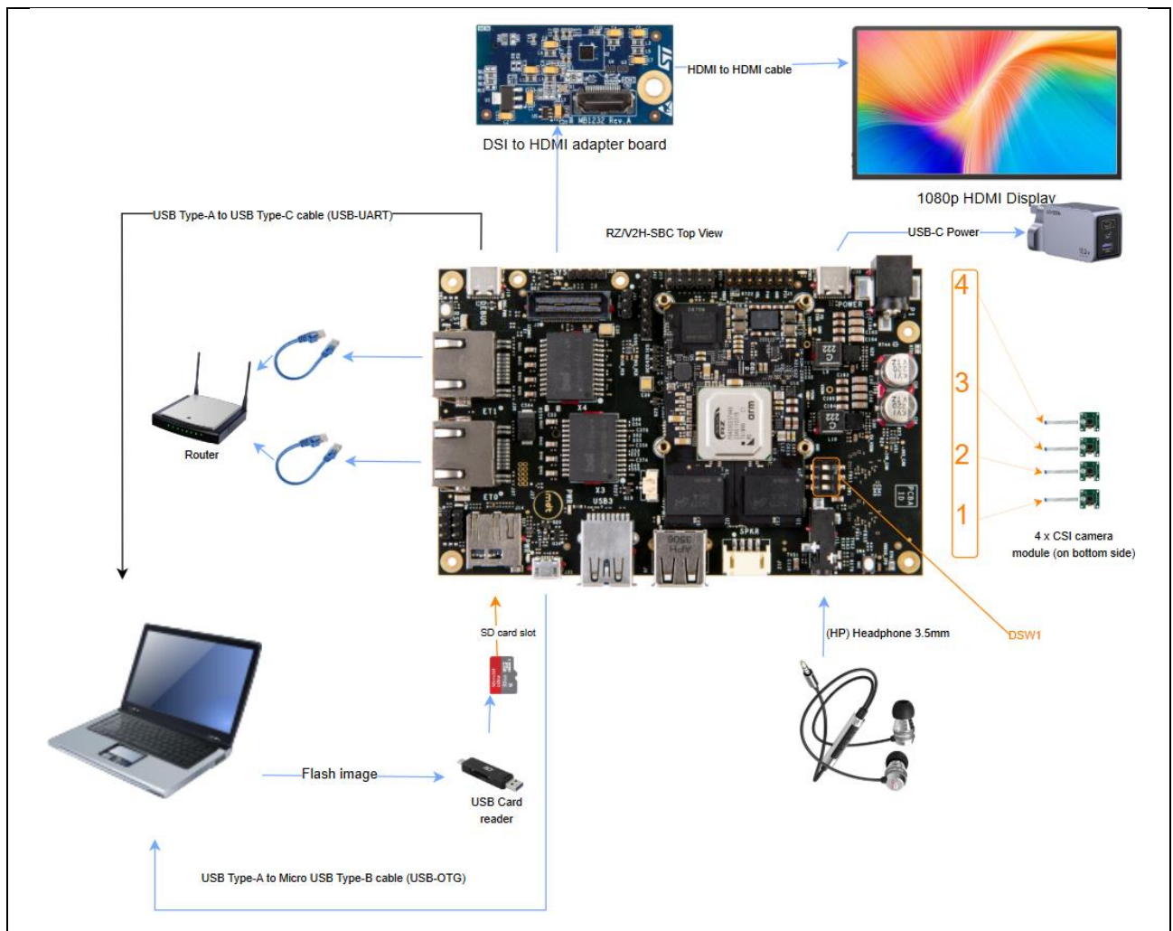
Figure 36. Complete setup for IMDT-V2H-SBC board
