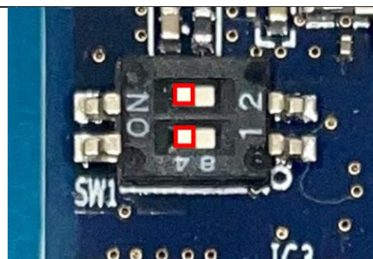
Figure 23. Enable SD slot CN3 with normal operation
