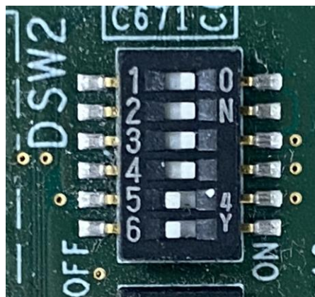
Figure 52. DSW2 - Audio Clock / Utility DIP
