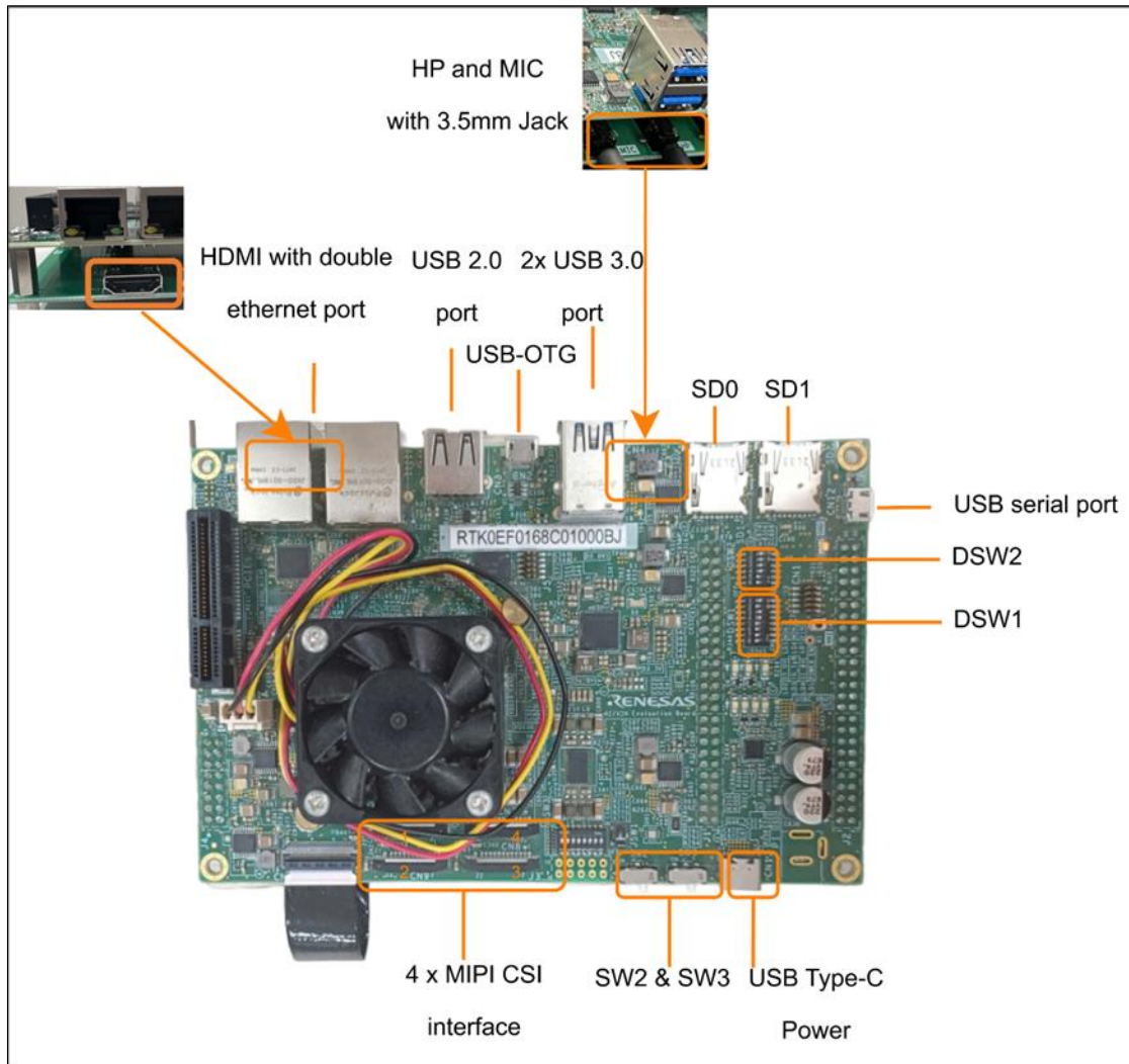
Figure 25: RZ/V2H-EVK Overview of Connectors
