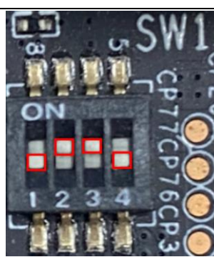
Figure 43. SW1 – eMMC Boot Mode
