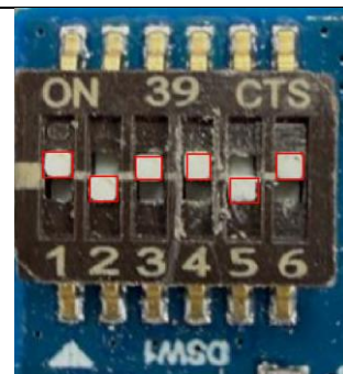
Figure 55. DSW1 – eSD Boot Mode
