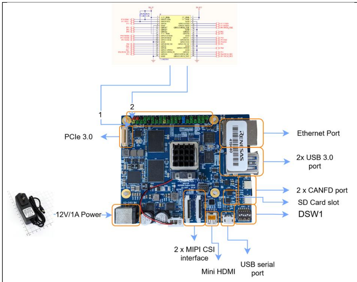
Figure 29. RZ/V2H-RDK - Overview of Connectors
