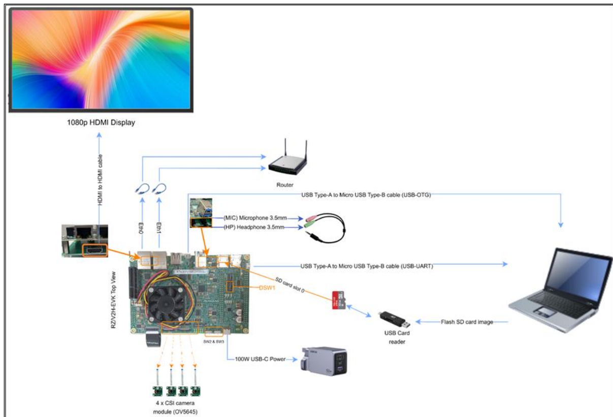
Figure 28: Complete setup for RZ/V2H-EVK board
