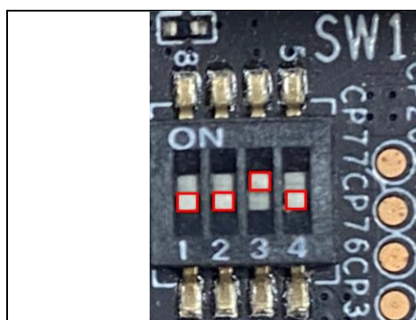
Figure 42. SW1 – QSPI Boot Mode
