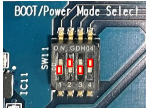
Figure 39. SW11 SCIF Download Mode - RZ/G2L-EVK & RZ/V2L-EVK
