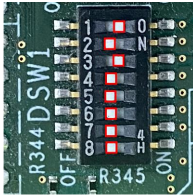
Figure 27. RZ/V2H-EVK xSPI boot mode
