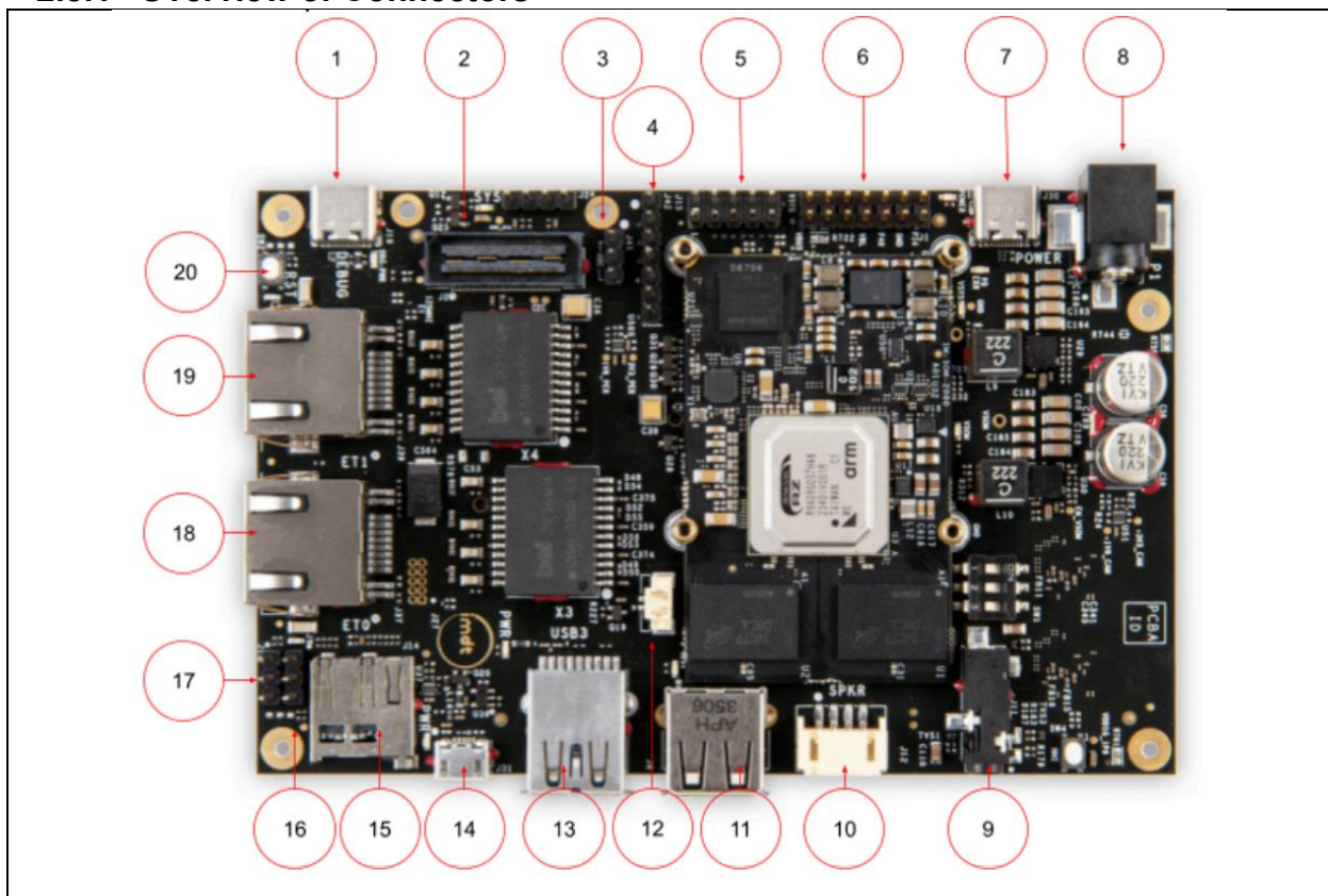
Figure 33. IMDT-V2H-SBC Top view
