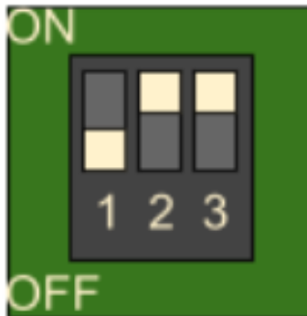
Figure 35. IMDT-V2H-SBC xSPI boot switch
