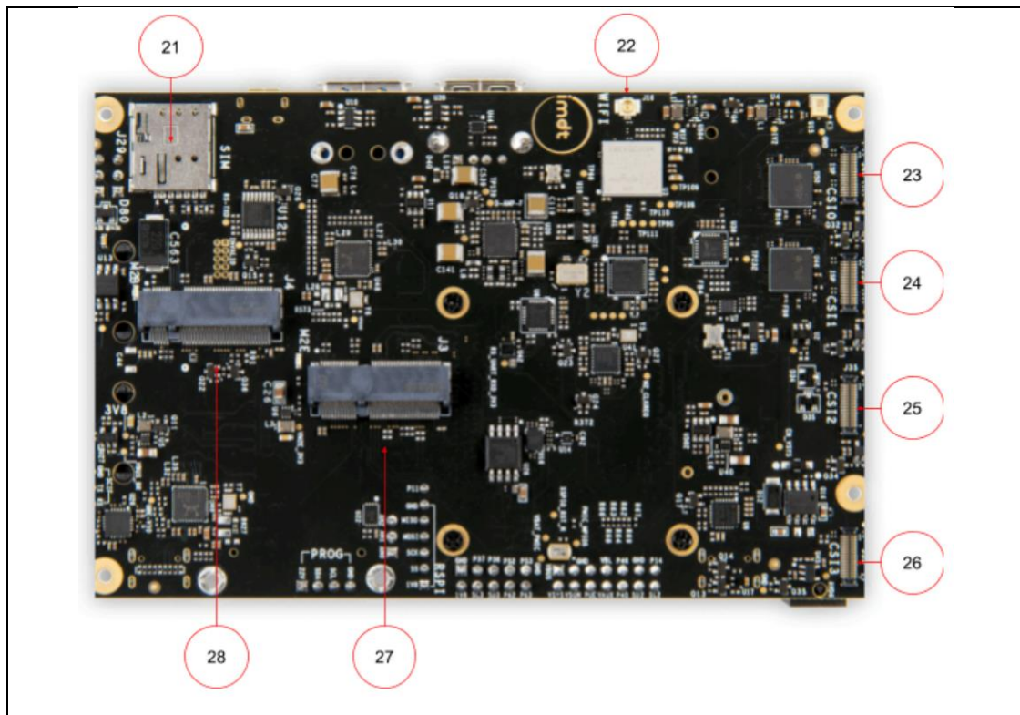
Figure 34. IMDT-V2H-SBC Bottom view
