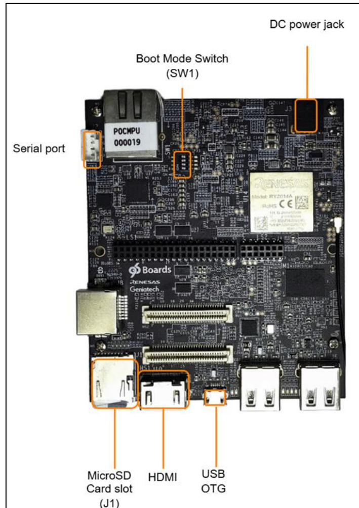
Figure 16. Essential minimum interfaces for RS-G2L100
