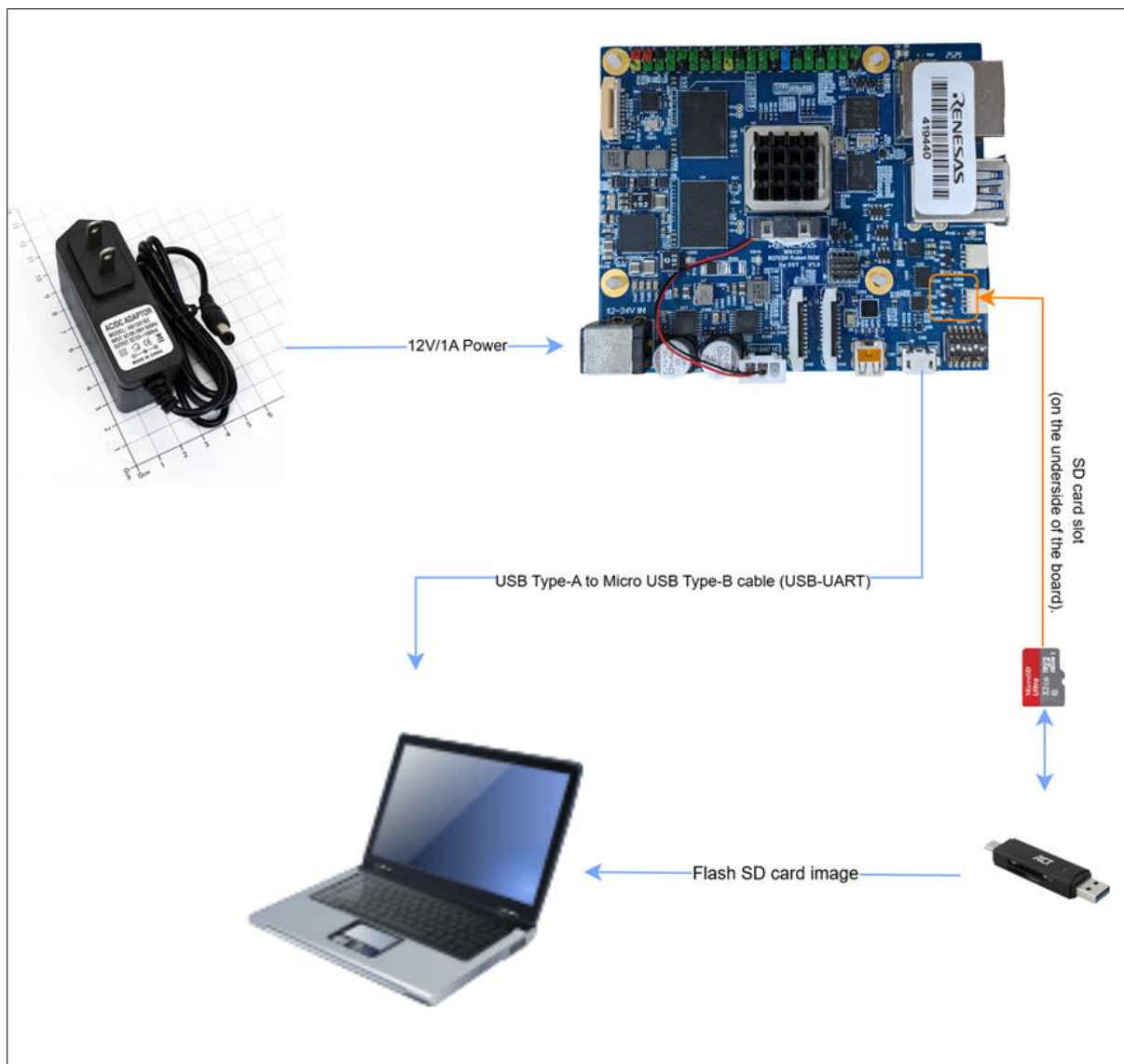
Figure 30. Essential minimum interfaces for RZ/V2H-RDK
