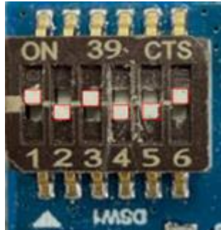
Figure 31. RZ/V2H-RDK xSPI boot switch
