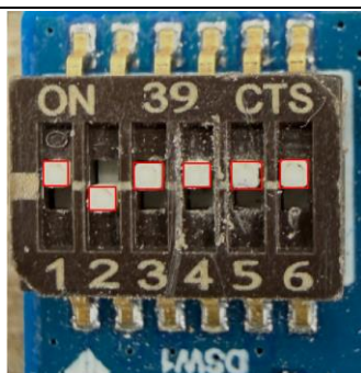
Figure 53. DSW1 - eMMC Boot Mode
