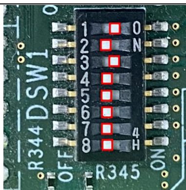
Figure 50. DSW1 - xSPI Boot Mode
