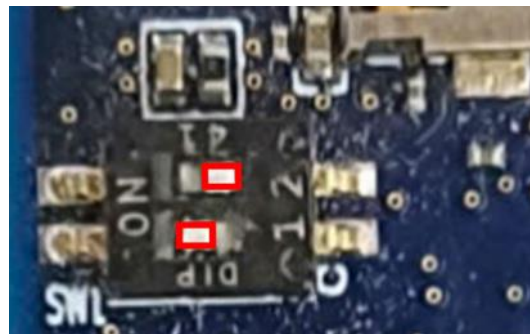
Figure 40. SW1 Settings for eMMC Boot - RZ/G2L-EVK & RZ/V2L-EVK
