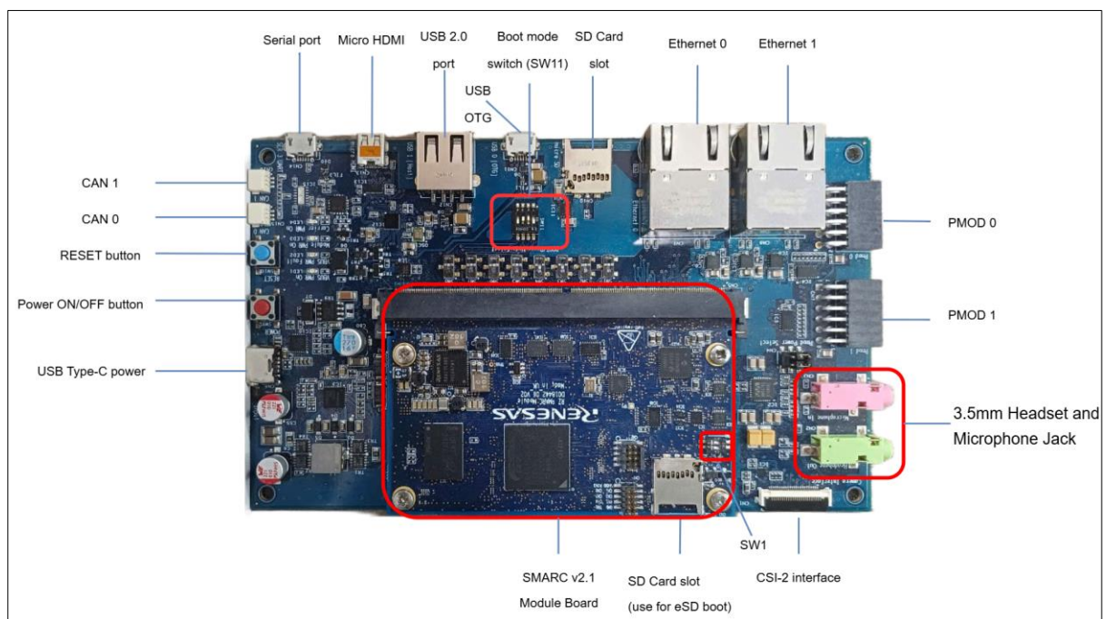
Figure 19: Overview of Connectors - RZ/G2L-EVK & RZ/V2L-EVK
