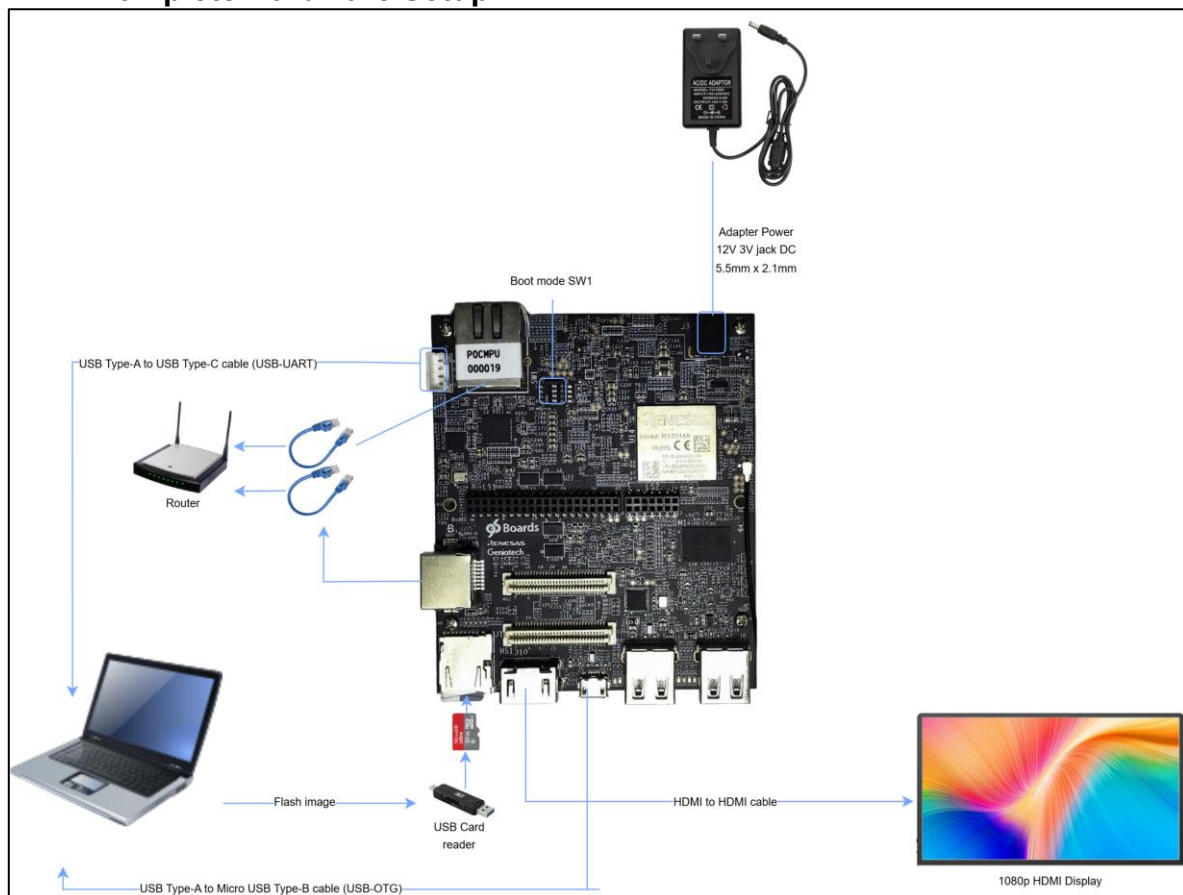
Figure 18. Complete setup for RS-G2L100
