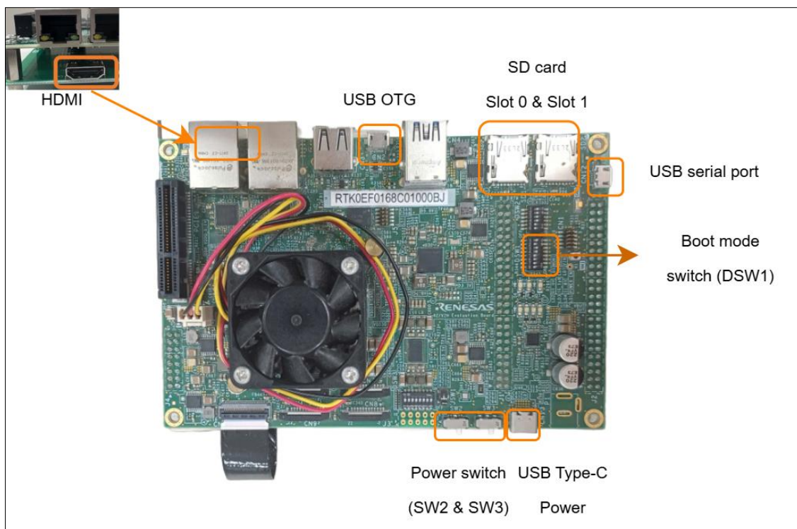
Figure 26: Essential minimum interfaces for RZ/V2H-EVK
