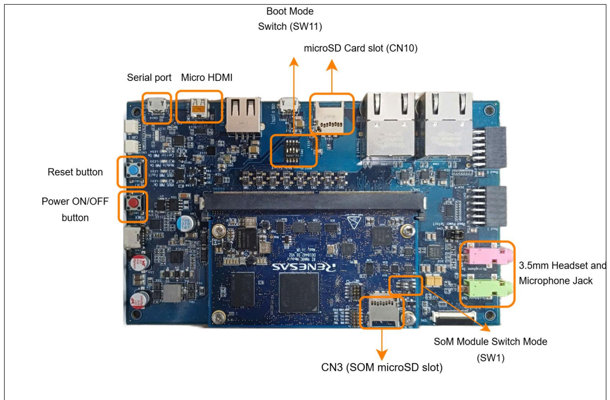
Figure 20. Essential minimum interfaces for RZ/G2L-EVK & RZ/V2L-EVK
