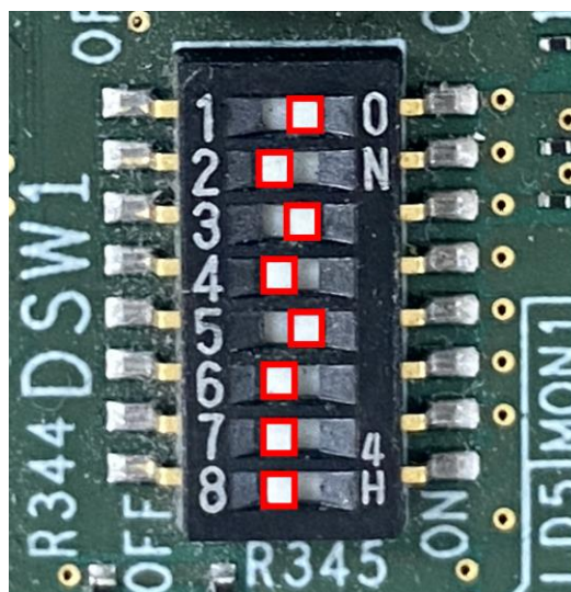
Figure 41. DSW1 - SCIF Boot Mode
