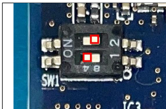
Figure 22. eMMC selection with normal operation
