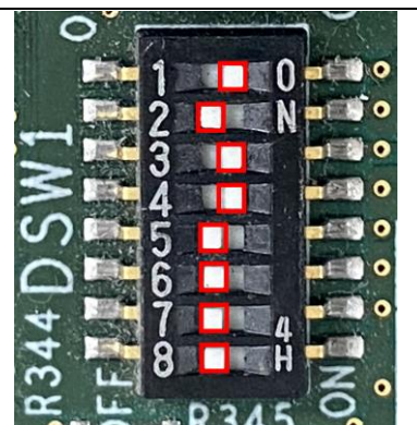
Figure 51. DSW1 - eSD Boot Mode
