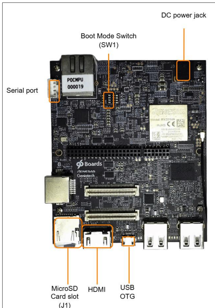
Figure 15. Overview of Connectors - RS-G2L100
