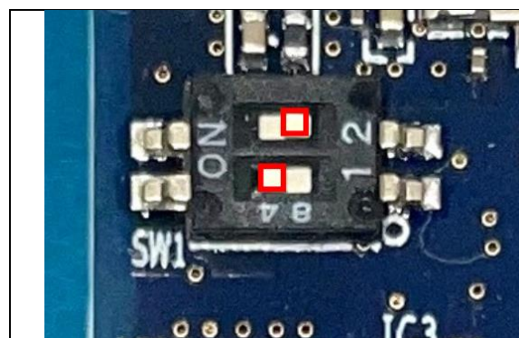
Figure 47. eMMC selection with normal operation
