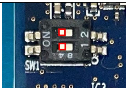
Figure 48. Enable SD slot CN3 with normal operation
