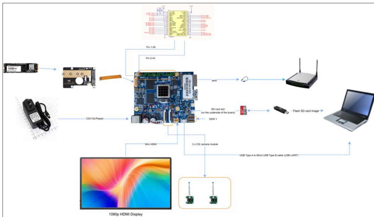
Figure 32. Complete setup for RZ/V2H-RDK board
