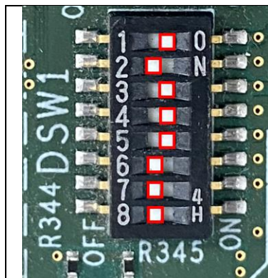
Figure 49. DSW1 - eMMC Boot Mode
